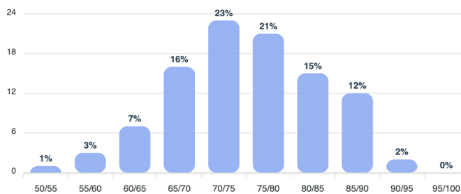
Calibres (724 fruits)
